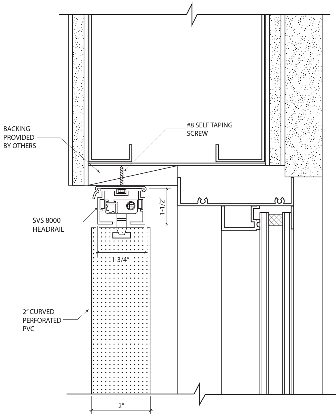
1 TYPICAL FIXED WINDOW HEAD 1/2 FULL SCALE
