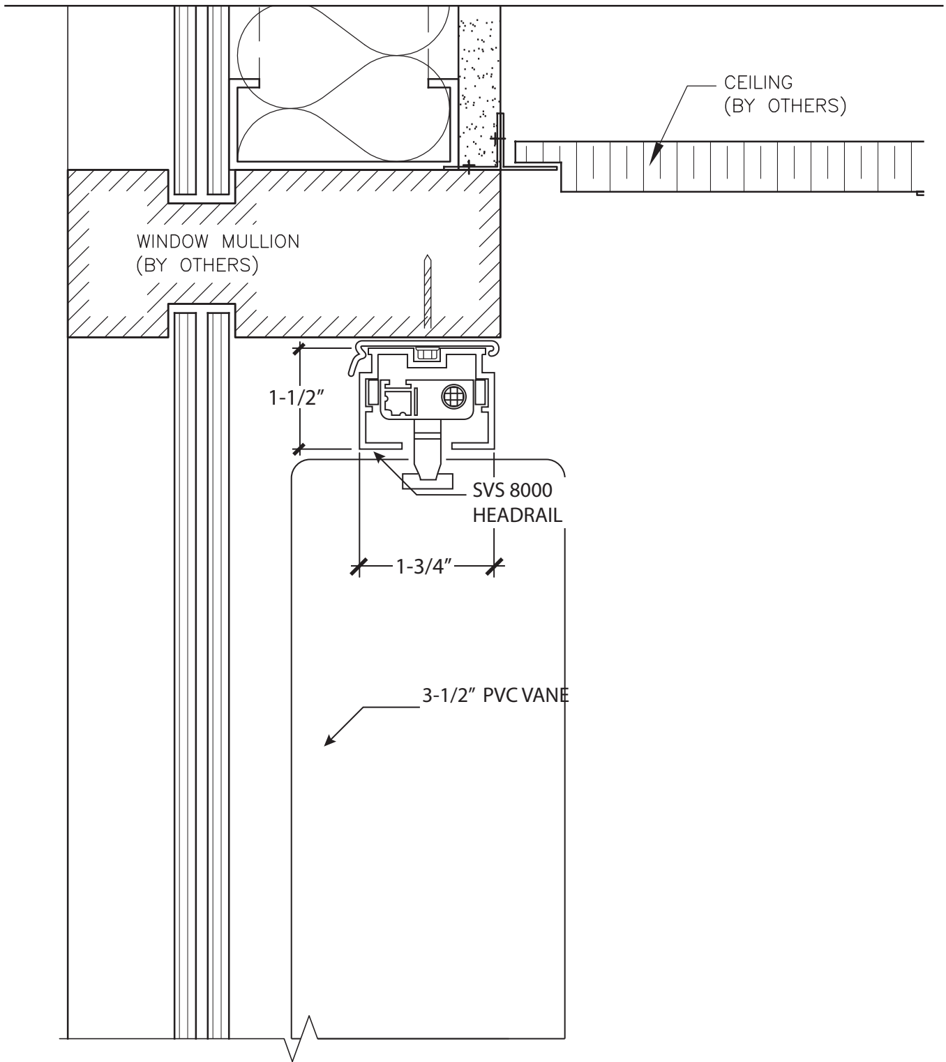
1 TYPICAL SECTION
