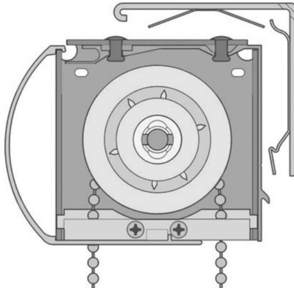
Round Front Fascia with optional Back Fascia – Profile Detail
